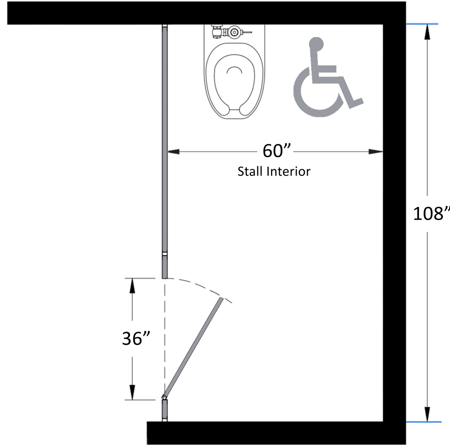
Bathroom Partitions - 1 Stall Alcove Right Hand ADA SKU: ALIC1RADA Standard Dimensions
